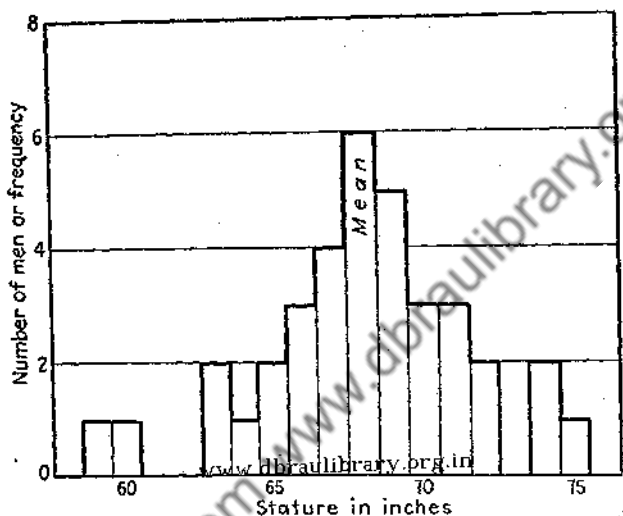
Fig. 1A.—Frequency diagram for data of Table 2.
