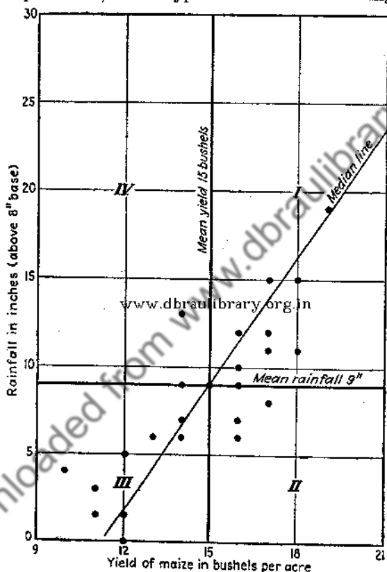
FIG. 6.—Dot diagram for rainfall and yield of maize over a 25-year period.
