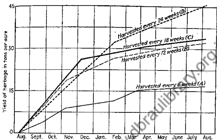
Fig. 2A.—Yields of herbage from four different harvesting rotations, over a period of twelve months. www.dbraulibrary.org.in
