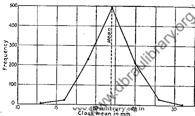
Fig. 5B.—Frequency diagram for length of cacao beans arranged in 3-mm. classes.
