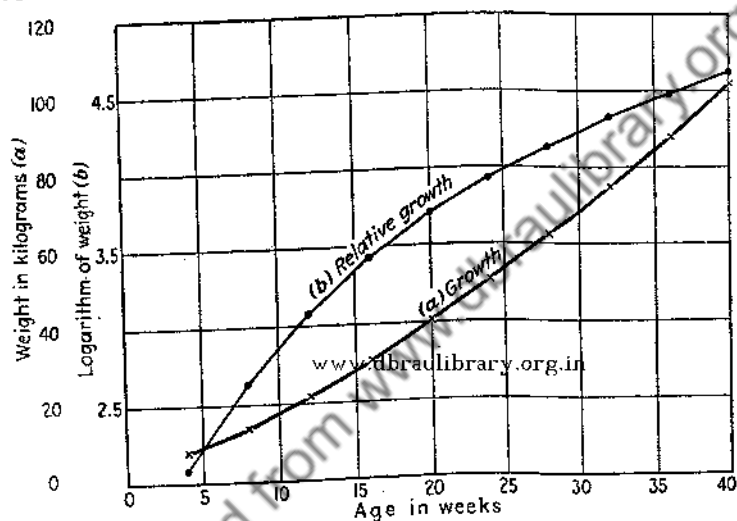
FIG. 4A.—Growth curves from a young pig.
